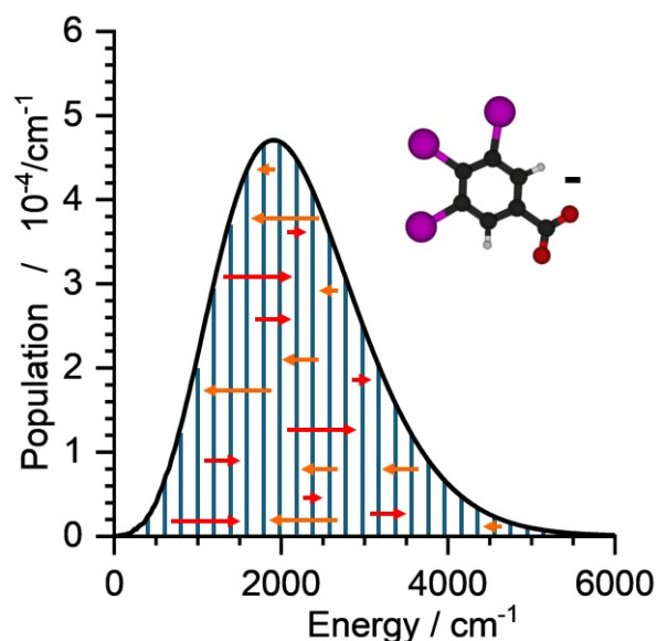
Figure 7: Single Well without dissociation: Population for \text{C}_6\text{H}_2\text{I}_3\text{COO}^- at 300 K in stationary state. Red arrows indicate photon absorption, orange arrows photon emission. Both processes shift population from one energy bin to another. In the stationary state, these shifts exactly cancel out.
