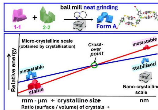
Figure 29 Stabilization of Form A of 1-2 under NG ball-milling conditions. (a) Disulfide exchange scheme under NG conditions. (b) Nanosizing-induced stability crossover: Form B, stable at μm+ sizes, becomes metastable at the nanoscale, while Form A, metastable at μm+ sizes, becomes stable at the nanoscale. 51 Adapted from Navrotsky's work on iron oxyhydroxide. 58
