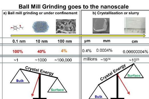
Figure 28 Effect of crystal size on polymorph formation. (a) Ball milling produces nanocrystals with significant surface contributions; (b) Solution or slurry crystallization generates μm–cm crystals where surface effects are negligible, so bulk stabilization dominates. Calculations by Aurora Cruz Cabeza.
