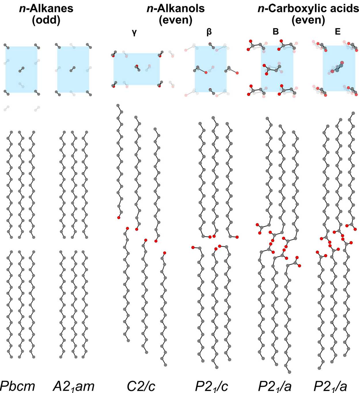
Fig. 3 Diagrams depicting the molecular packing arrangement in reported unit cells for odd- n long-chain alkanes ( n -alkanes), even- n primary alcohols ( n -alkanols), and even- n fatty acids ( n -carboxylic acids). The molecules are shown viewed along the long-axis of the molecule ('down-chain') at the top and viewed side-on below. A blue box indicates the polyethylene-like unit cell (sub-cell) for each structure. The space groups of each structure are given at the bottom. Carbon atoms are shown in grey, and oxygen atoms are shown in red. Hydrogen atoms are omitted for visual simplicity. The chain lengths shown ( n = 18 – 19 ) are shortened for visual clarity relative to the longer chains present in leaf waxes ( n \sim 21 – 35 for n -alkanes).
