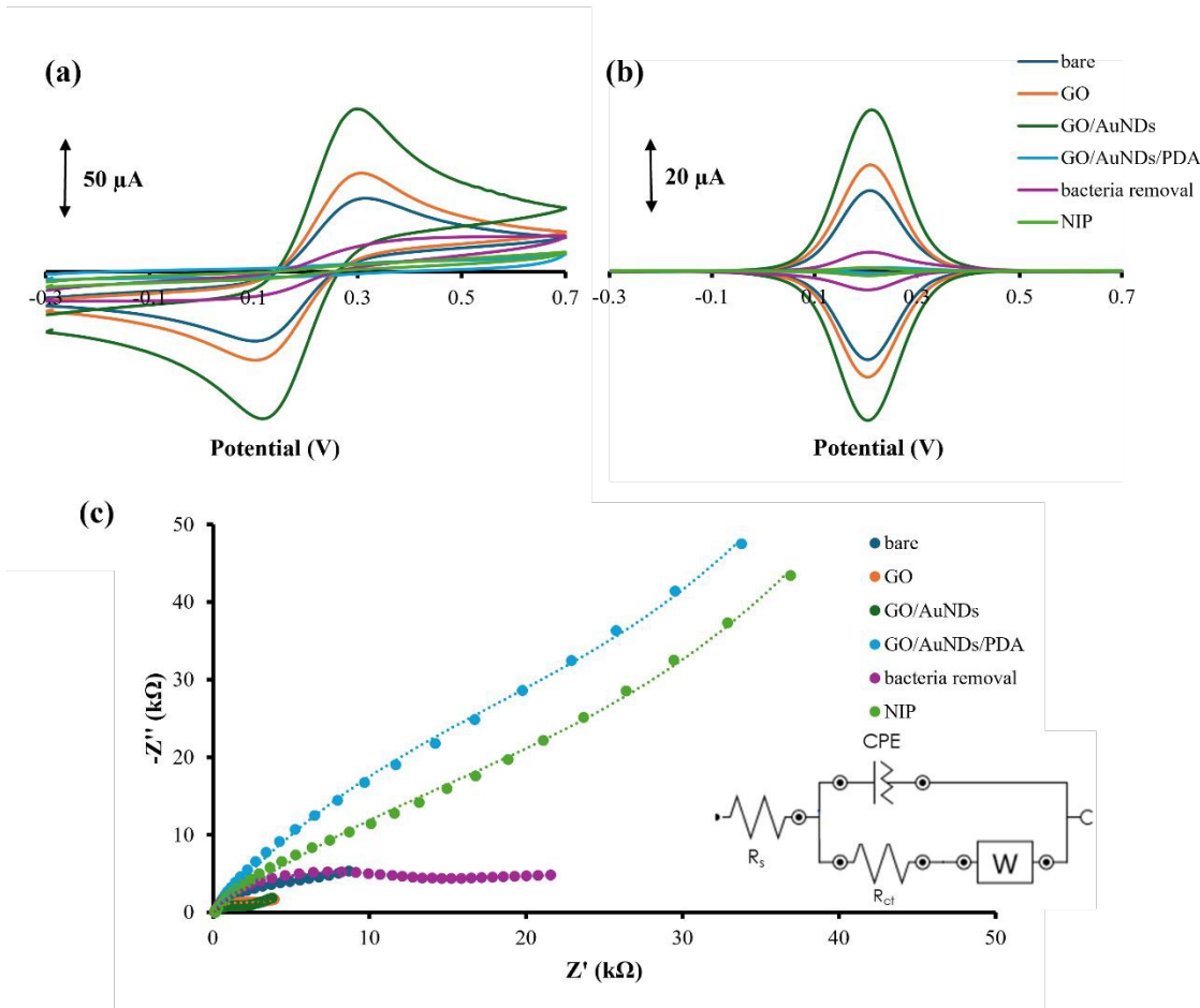
Figure 3. (a) CV (from -0.3 to 0.7 V, 100 mV/s scan rate) and (b) DPV (from -0.3 to 0.7 V and from 0.7 to -0.3 V with 100 scan rate mV/s, 5 mV step, 25 mV modulation amplitude) of GO/AuNDs/PDA GCE measured in 5 mM [\text{Fe}(\text{CN})_6]^{3-/4-} in 0.1 M \text{KNO}_3 vs. Ag/AgCl reference electrode, (c) Nyquist plots of GO/AuNDs/PDA GCE measured in 5 mM [\text{Fe}(\text{CN})_6]^{3-/4-} in 0.1 M
