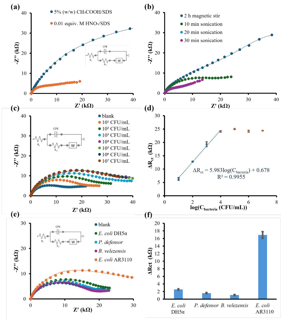
Figure 4. Bacteria template removal studies using (a) 5% (w/w) \text{CH}_3\text{COOH}/\text{SDS} vs. 0.01 M equiv. M \text{HNO}_3/\text{SDS} and (b) 0.01 M equiv. M \text{HNO}_3/\text{SDS} with 2 h of magnetic stirring vs. 10, 20, and 30 min of sonication. (c) Nyquist plots of GO/AuNDs/PDA GCE with 10 cyclise of polymerization after incubation in different concentrations of E. coli , fitted with the modified Randles equivalent circuit (inset), and (d) the plot of \Delta R_{ct} vs. log concentration of E. coli ( n = 3 ). (e) Nyquist plots of GO/AuNDs/PDA GCE after incubation in 1.0 \times 10^3 CFU/mL of E. coli DH5 \alpha , P. defensor , B. velezensis , and E. coli AR3110, measured under the same conditions ( n = 3 ), and (f) bar chart of corresponding \Delta R_{ct} . Nyquist plots were measured in 5 mM [\text{Fe}(\text{CN})_6]^{3-/4-} .
