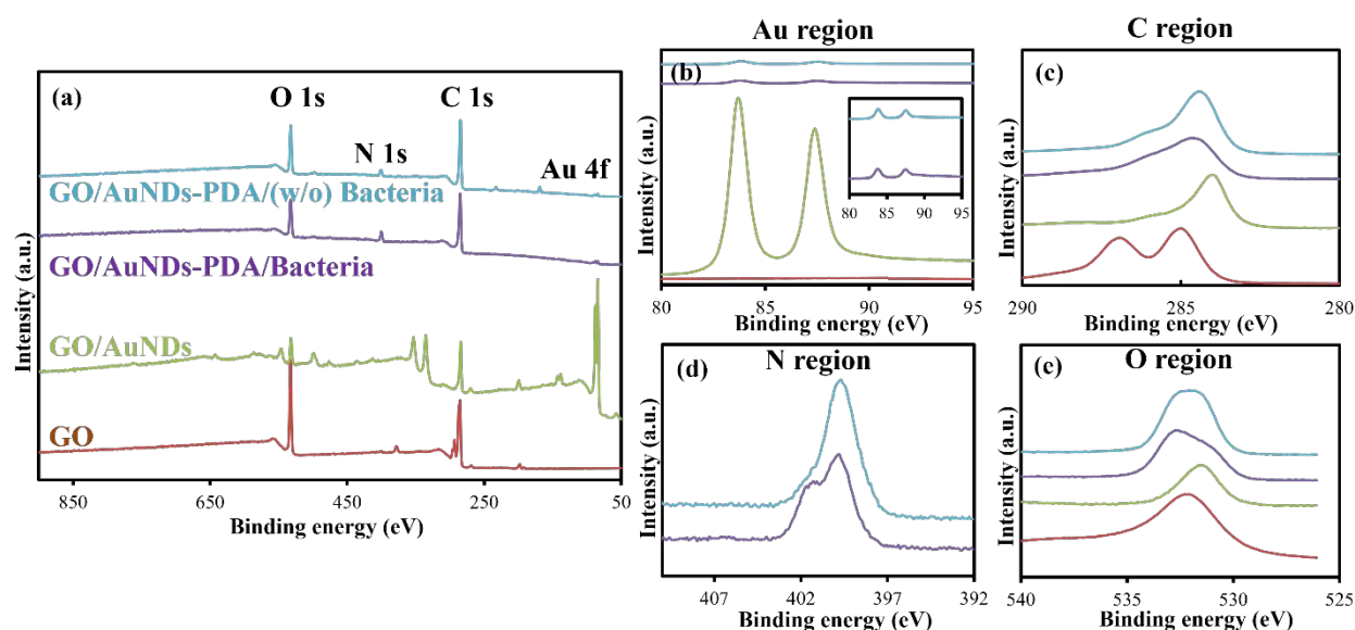
Figure 2. (a) XPS survey for the step-by-step modification of GCE with GO, GO/AuNDs, GO/AuNDs/PDA/Bacteria, and GO/AuNDs/PDA/(w/o, without) Bacteria, where bacteria were washed off, and stack plot of in survey of the (b) Au region, (c) C region, (d) N region, and (e) O region.
