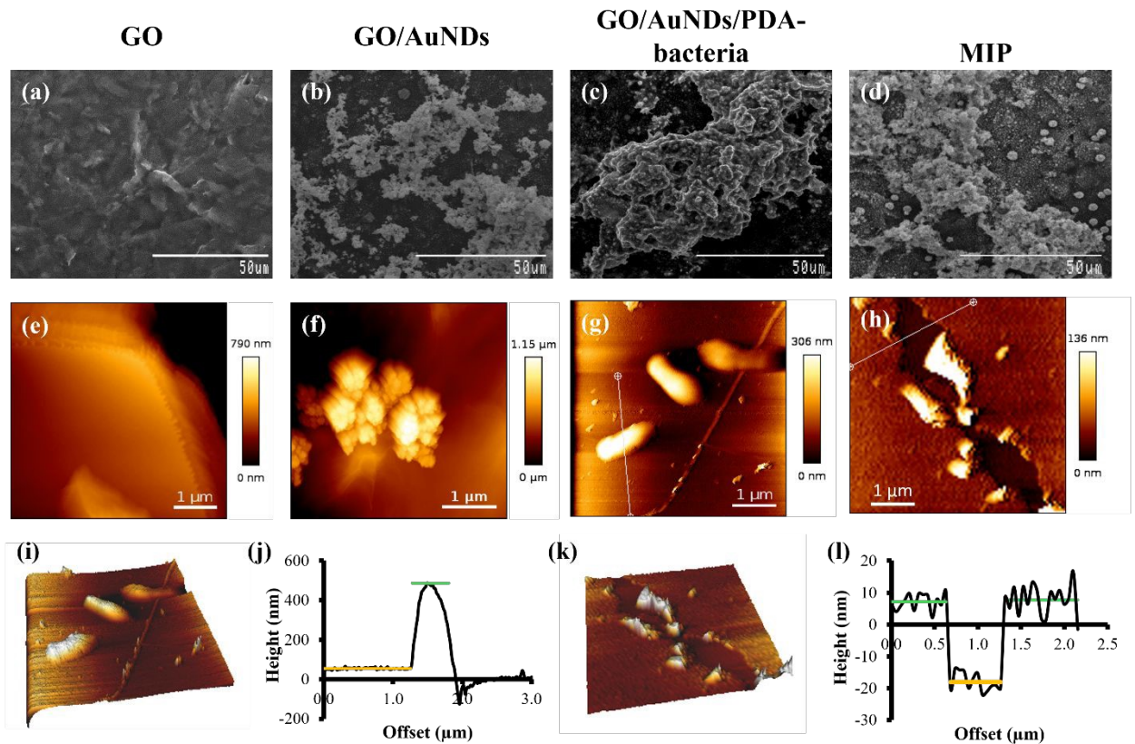
Figure 1. SEM images for modified GCEs with (a) GO, (b) GO/AuNDs, (c) GO/AuNDs/PDA-Bacteria, and (d) MIP. 2D AFM images of (e) GO, (f) GO/AuNDs, (g) bacteria trapped in the PDA film, (h) the MIP pattern observed after the removal of bacteria, and (i) a 3D AFM image of bacteria trapped in the PDA film with (j) the cross-section analysis of bacteria height, and (k) a 3D AFM image of the MIP pattern after the removal of the bacteria with (l) the cross-section analysis of an imprinted cavity.
