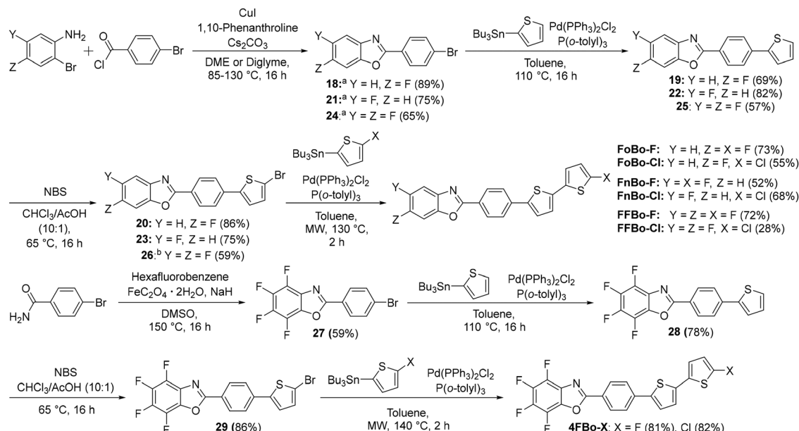
Scheme 3 Synthetic route for core-only calamitics with the benzene ring of benzoxazole partially or fully fluorinated, consisting of FoBo-X , FnBo-X , FFBo-X and 4FBo-X ( X = F or Cl ). 18 was achieved using DME at reflux, while 21 and 24 were achieved using diglyme at 120 °C and 130 °C, respectively. b Reaction conditions vary from what is shown, as DMF/acetic acid (10 : 1) at 85 °C was used instead.
