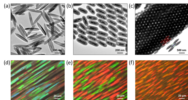
Fig. 2 Magnetic assembly of nanorods into tetragonal photonic crystals. TEM images of (a) \text{FeOOH} nanorods, (b) \text{Fe}_3\text{O}_4@/\text{SiO}_2 nanorods, and (c) the tetragonal photonic crystals. Inset in (c) shows one unit cell of the body-centered tetragonal crystals. Nanorods in one unit cell are highlighted in dashed red ellipses. Optical microscopy images of the responsive photonic crystals under different magnetic field directions: (d) 0^\circ , (e) 30^\circ , and (f) 50^\circ . The external magnetic field directions are defined by the angle between the field direction and the horizons in the incident planes as illustrated in Fig. S2d.
