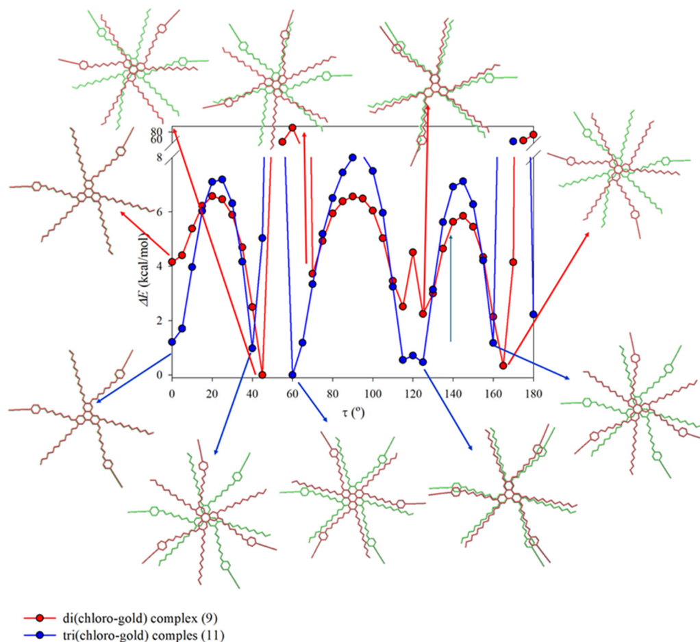
Fig. 8 Relative energy ( \Delta E ) evolution as a function of the azimuthal angle ( \tau ) between triphenylene cores. Inter-molecular \pi -stacking distances have been fixed according to experimental data from X-ray diffraction studies. \Delta E values were calculated with respect to the minimum energy situation for each complex ( \tau = 45^\circ and 60^\circ for the di(chloro-gold) and tri(chloro-gold) complexes, respectively). Representations of two stacked molecules of di(chloro-gold) and tri(chloro-gold) complexes ( 9 and 11 , respectively, where both molecules are highlighted in different colours) corresponding to configurations with minimal energy as a function of the azimuthal angle ( \tau ) are also displayed. H atoms are omitted.
