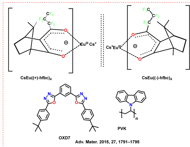
Scheme 7 Chemical structures of the ligands and Ln complexes \text{CsEu}(\text{hfbc})_4 . 54 OXD7 = 1,3-bis[2-(4- tert -butylphenyl)-1,3,4-oxadiazacyclononane-5-yl]benzene; PVK = polyvinylcarbazole.
