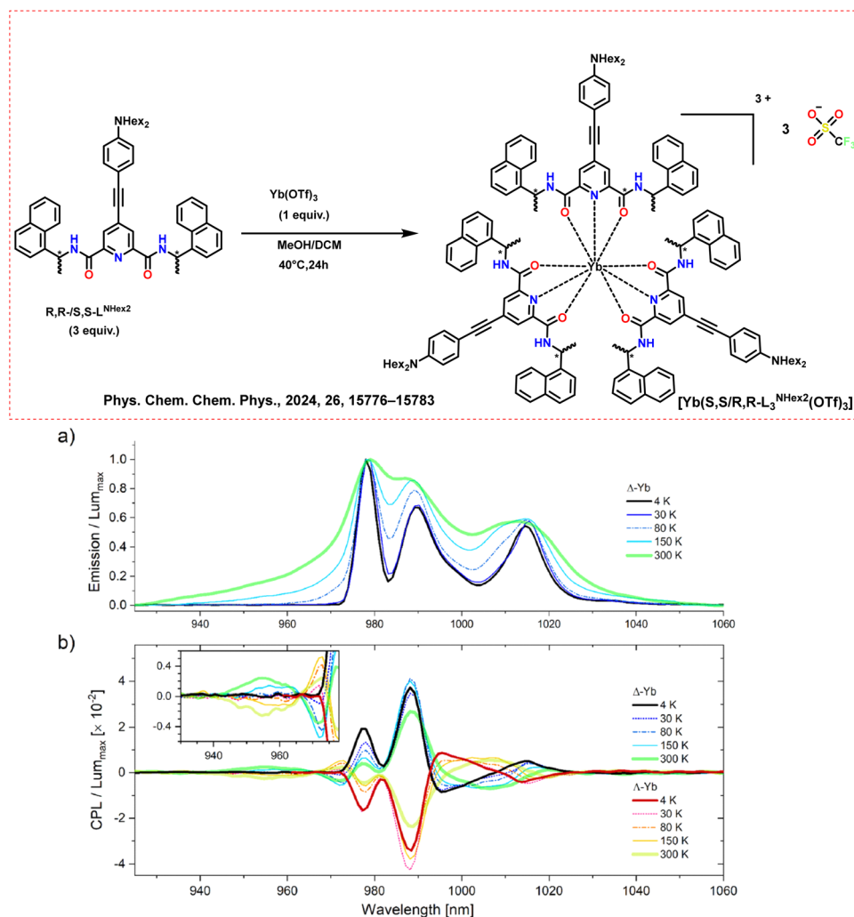
Scheme 43 (Above) Chemical structures of the ligands and Ln complexes [Yb(S,S/R,R-L NHHex 2 3 (OTf) 3 ], adapted from ref. 103. (Below) Variable temperature spectra of the two Yb 3+ complexes in PDMS at 4, 30, 80, 150 and 300 K. (a) Variable temperature-luminescence spectra for D-Yb. (b) Variable temperature-CPL spectra. Inset shows the enlarged region of hot bands. Reproduced from ref. 103 with permission from the Royal Society of Chemistry, copyright [2024]. 103
