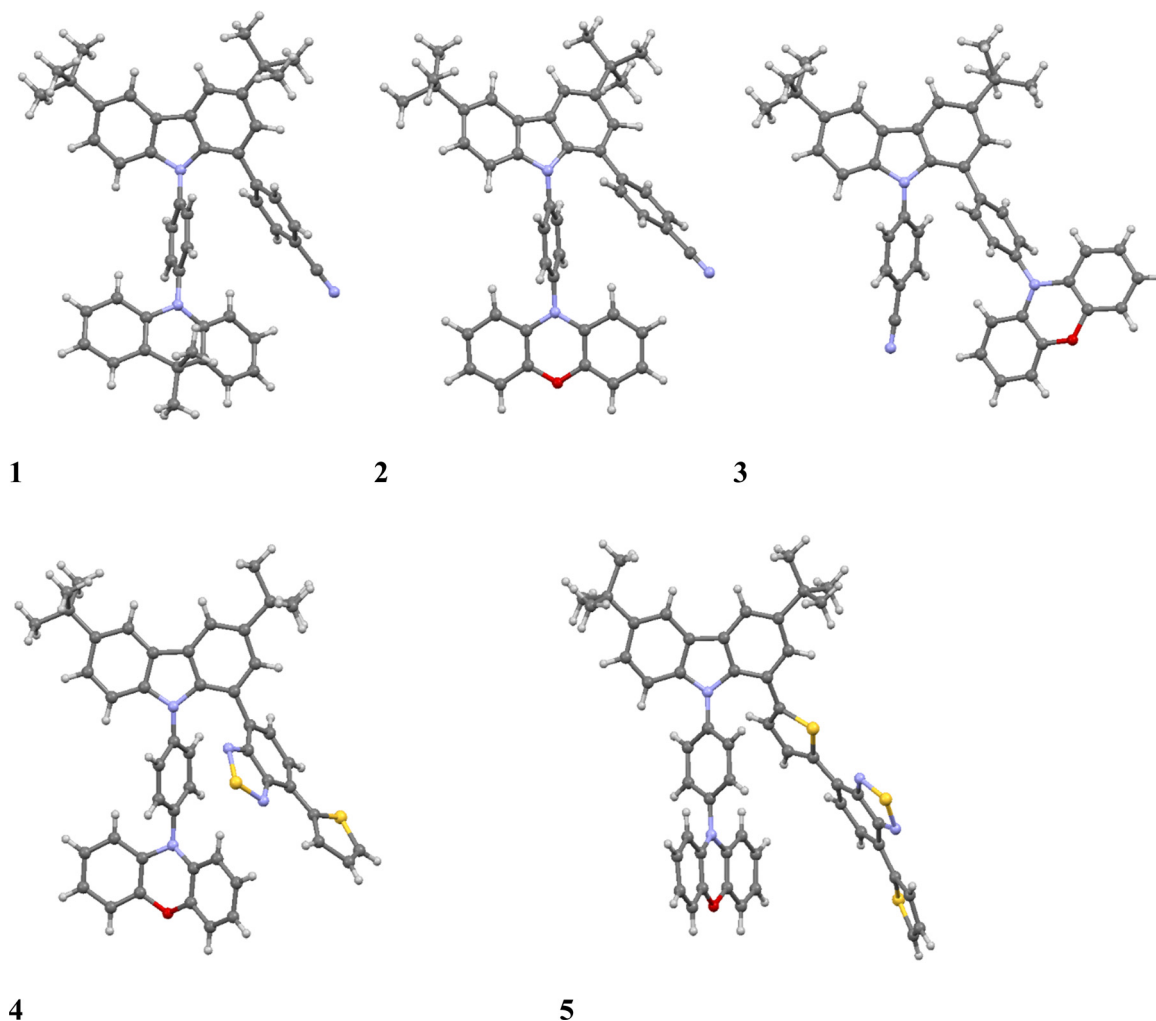
Fig. 3 Molecular structures of 1–5 . In the case of disorder, the parts with bigger occupancies are shown. The figures with all details (disorder and ADPs) are given in (ESI†).
