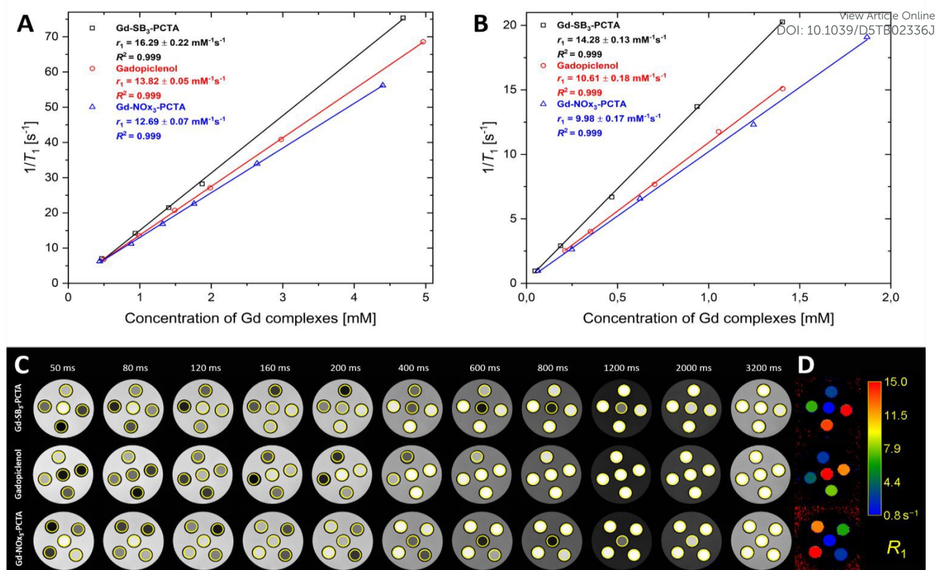
Fig. 3 (A) Longitudinal relaxivity ( r_1 ) determined from plotting the reciprocal relaxation time 1/T_1 versus the concentration of Gd-SB 3 -PCTA 11a , Gd-NOx 3 -PCTA 12a and gadopichlenol 3 in H 2 O at 37 °C and 1.4 T (60 MHz) (B) Longitudinal relaxivity ( r_1 ) determined from plotting the reciprocal relaxation time 1/T_1 versus the concentration of Gd-SB 3 -PCTA 11a , Gd-NOx 3 -PCTA 12a and gadopichlenol 3 in H 2 O at room temperature and 7 T (300 MHz) (C) Representative MR images acquired at 7 T at multiple inversion times (TI) ranging from 50 ms to 3200 ms of Gd-SB 3 -PCTA 11a , Gd-NOx 3 -PCTA 12a and gadopichlenol 3 in a phantom holder and surrounded by water. Yellow circles represent the regions of interest for five different concentrations of each compound used for subsequent quantitative analysis. (D) Color-coded R_1 relaxation rate map acquired at 7 T with an inversion-recovery spin-echo sequence with multiple inversion time delays for five different concentrations of each compound.
