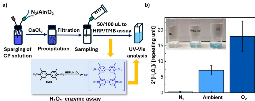
Fig. 2 (a) Scheme of the experimental procedure used for the autonomous production and quantification of \text{H}_2\text{O}_2 by P(2CAT-K); (b) oxidation level of P(2CAT-K) based on measured \text{H}_2\text{O}_2 concentration (multiplied by two) per number of polymer repeating unit obtained after exposing the same P(2CAT-K) aqueous nanodispersion to three different environments: \text{O}_2 , ambient air and \text{N}_2 atmosphere. Inset: Color of the filtrated solutions after addition to the HRP/TMB assay. The blue color is related to the charge-transfer complex formed by TMB in the presence of HRP enzyme and \text{H}_2\text{O}_2 .
