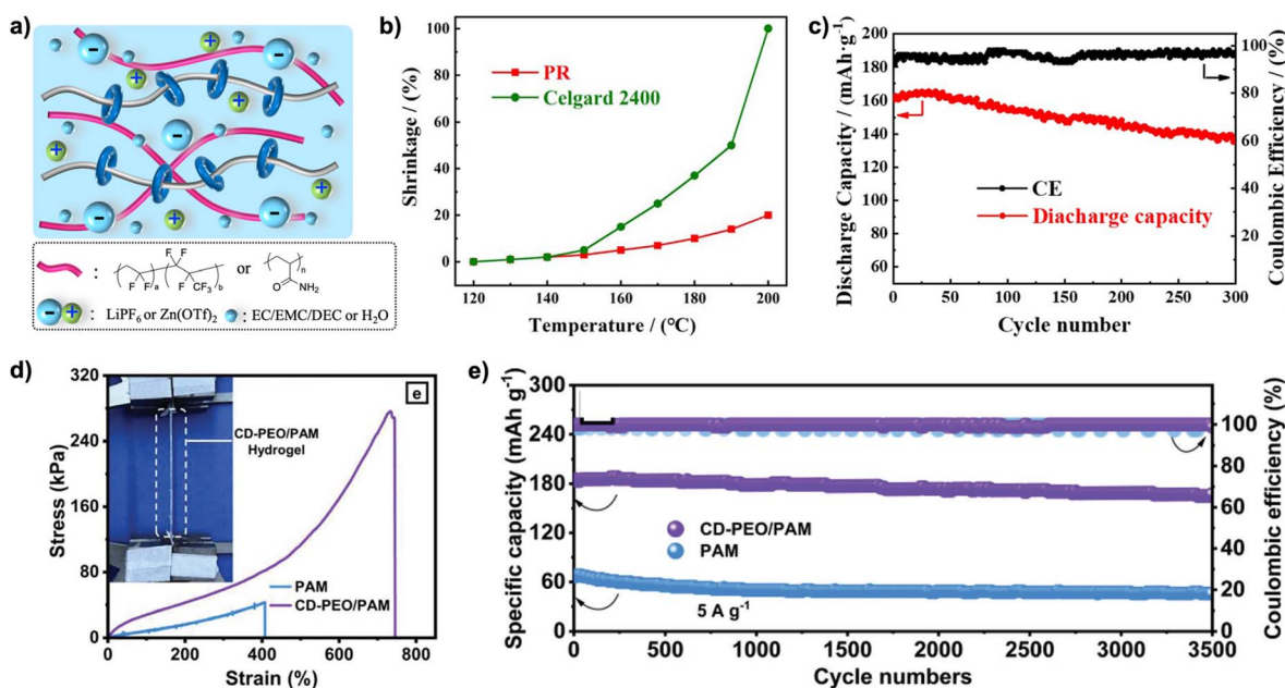
Fig. 8 (a) Composite gel electrolyte consisting of pseudo-PR and PVDF-HFP or PAM. (b) A pseudo-PR composite gel electrolyte exhibited higher thermal stability than a commercial Celgard 2400 membrane, and (c) its use in an NMC532||Li full battery enabled 86% capacity retention after 300 cycles at 0.5C. A CD-PEO/PAM composite electrolyte showed higher (d) mechanical toughness and (e) cycling capacity in a La- \text{V}_2\text{O}_5 ||Zn battery than the PAM gel electrolyte. (b and c) are reproduced from ref. 68 with permission from Springer, copyright 2022. (d and e) are reproduced from ref. 69 with permission from Wiley, copyright 2023.
