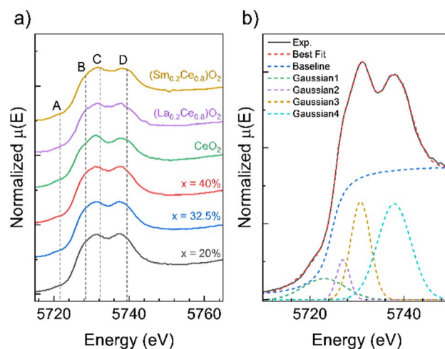
Fig. 5 (a) Ce L_3 absorption edge of Ce in \text{Ce}_x(\text{SmPrLaY})_{1-x}\text{O}_{2-d} and measured standards, peaks used for fitting labeled A–D and are defined in the text. (b) Example of fitting procedure for the Ce L_3 edge on \text{CeO}_2 .
