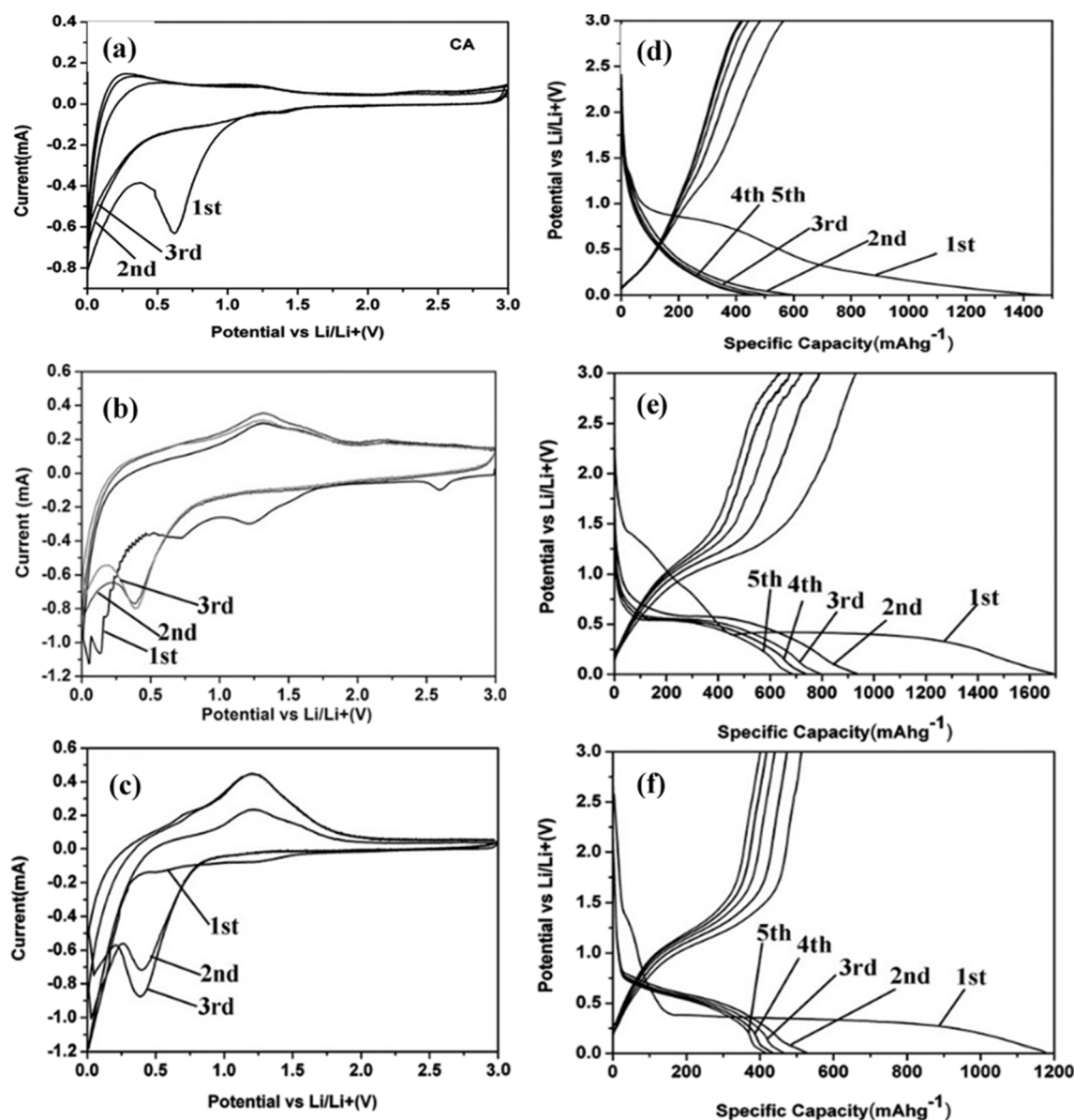
Fig. 9 CV curves of the first three cycles for (a) CA, (b) the 50% ZMO/CA hybrid, and (c) pure ZMO samples at a scan rate of 0.1 mV s -1 in the voltage range of 0.01–3.0 V. Initial charge–discharge curves of (d) CA, (e) the 50% ZMO/CA hybrid, and (f) pure ZMO samples at a current density of 100 mA g -1 . Reproduced from ref. 98 with permission from Wiley Online Library, copyright 2014.
