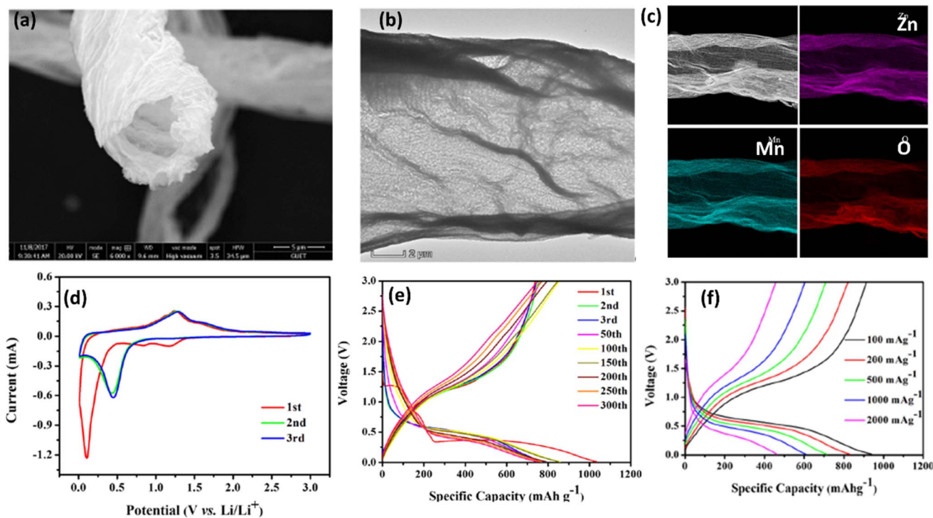
Fig. 11 ZMO microtubules (ZMO-MTs): (a) SEM image, (b) HR-TEM image, (c) elemental mapping, (d) CV curves at a scan rate of 0.1 \text{ mV s}^{-1} within the voltage range of 0.01–3.0 V, (e) GCD profiles after different cycles, and (f) GCD profiles at various current densities ranging from 100 to 2000 \text{mA g}^{-1} . Reproduced from ref. 95 with permission from ACS, copyright 2018.
