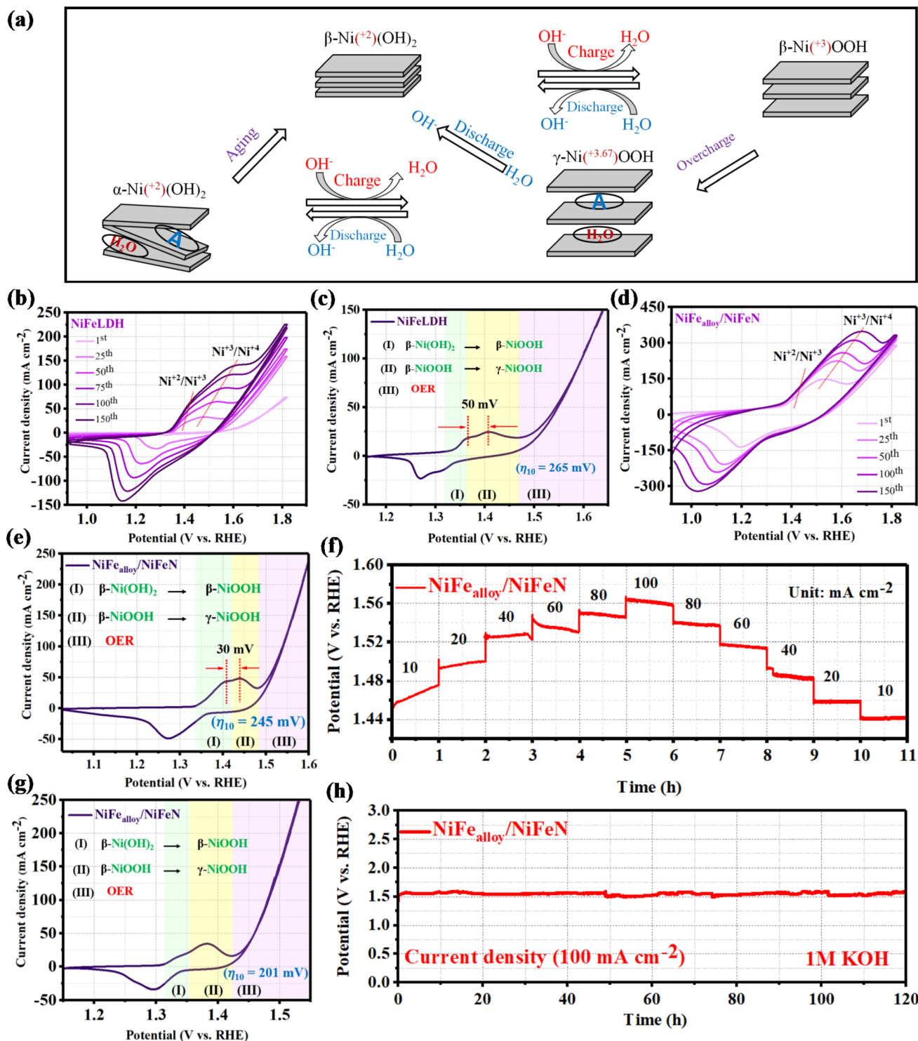
Fig. 5 (a) Overview of the transformations between distinct phases of Ni(OH) 2 and NiOOH. Note that A represents the possible anion of the acid (e.g., NO 3 -2 ; SO 4 -2 ; PO 4 -3 ) that can be incorporated between the layer of hydroxide. Electrochemical surface reconstruction of NiFeLDH and NiFe alloy /NiFeN: (b) cyclic voltammetry curves of NiFeLDH in the potential range from 0.9 to 1.8 (V vs. RHE). (c) Steady-state performance curve of NiFeLDH after 150 cycles of CV activation. (d) Cyclic voltammetry curves of NiFe alloy /NiFeN in the potential range from 0.9 to 1.8 (V vs. RHE). (e) Steady-state performance curve of NiFe alloy /NiFeN after 150 cycles of CV activation. (f) Chronopotentiometry activation of NiFe alloy /NiFeN at different current densities ranging from 10 to 100 mA cm -2 . (g) Steady-state performance curve of NiFe alloy /NiFeN after chronopotentiometry activation. (h) Long-term stability test of NiFe alloy /NiFeN at a current density of 100 mA cm -2 .
