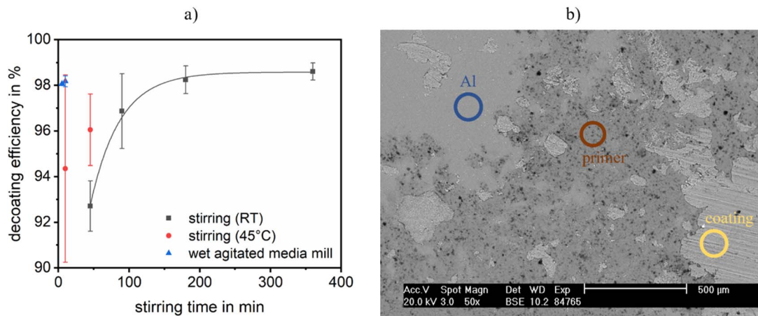
Fig. 7 Decoating results with (a) decoating efficiency at varying stressing times while using stirring (at room temperature and 45 °C) compared to the wet agitated media mill (b) surface of a cathode sheet particle that has been stirred for 360 min, where residues of the primer (red) and composite coating (yellow) can be seen on the aluminium foil (blue).
