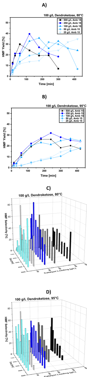
Fig. 6 Time resolved screening of the Amb15 catalyst loading between 10 g per L to 500 g per L for the dendroketo dehydration reaction to synthesize 4-HMF. (A) HMF yield at 100 g per L dendroketo loading and 80 °C, (B) HMF yield at 100 g per L dendroketo loading and 95 °C, (C) HMF reaction selectivity at 100 g per L dendroketo loading and 80 °C, (D) HMF reaction selectivity at 100 g per L dendroketo loading and 95 °C. HMF yields and selectivity were determined by ^1\text{H} -NMR analysis (error of \pm 5\% for the dendroketo quantification).
