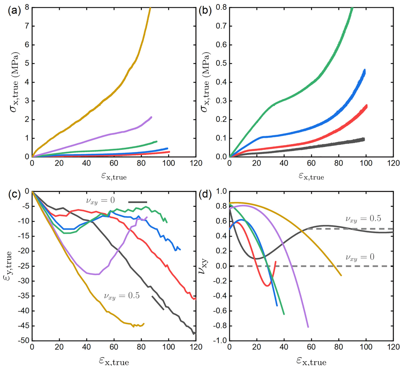
Fig. 5 Mechanical deformation behaviour of the LCEs where black = 1/16\times , red = 1/8\times , blue = 1/4\times , green = 1/2\times , purple = <
