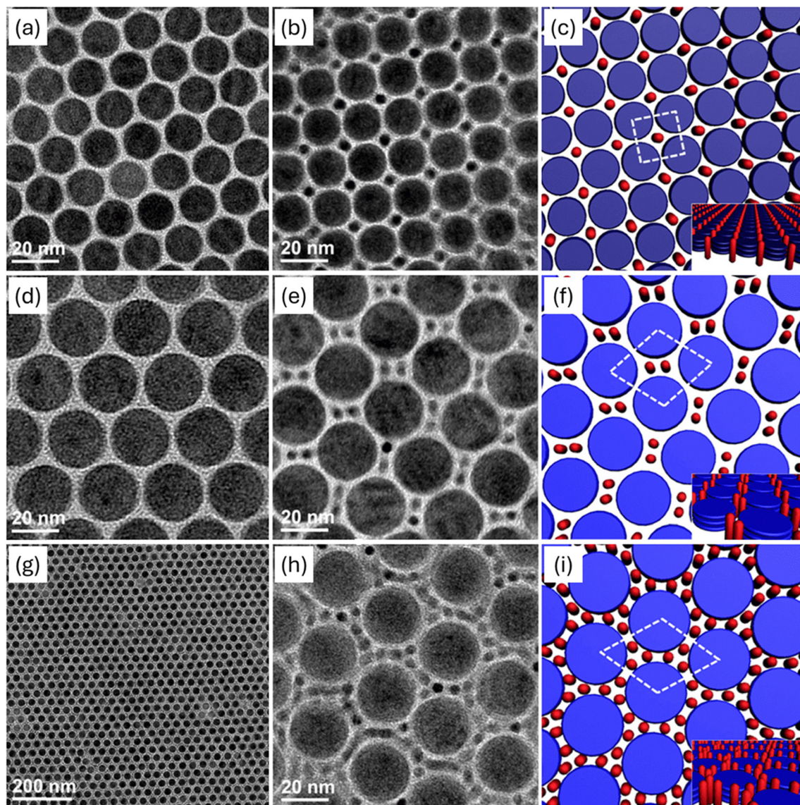
Fig. 26 Binary superstructures assembled from \text{LaF}_3 nanodisks and \text{CdSe/CdS} nanorods. TEM images of (a) a superstructure self-assembled from 13.2 nm \text{LaF}_3 nanodisks, (b) an LS-type binary superstructure, (d) a superstructure self-assembled from 22.3 nm \text{LaF}_3 nanodisks, (e) an \text{LS}_2 -type binary superstructure, and (g) and (h) an \text{LS}_6 -type binary superstructure. Structural models of (c) the LS-type binary superstructure, (f) the \text{LS}_2 -type binary superstructure, and (i) the \text{LS}_6 -type binary superstructure. Adapted with permission from ref. 235. Copyright 2015 American Chemical Society.
