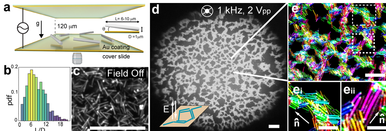
Fig. 1 (a) Scheme of the experimental setup, with a colloidal dispersion of SU8-rods sedimenting between two parallel electrodes. The spacing between the electrodes is 120 \mu\text{m} . The arrow pointing down indicates gravity acting on the sedimenting rods. (b) Normalized frequency of the aspect ratio of the colloidal suspension of rods ( L/D ) with a polydispersity \approx 20\% (c) Fluorescence microscopy image of a monolayer of SU-8 rods in the absence of an electric field. (d) Fluorescence microscopy of an interconnected network of SU-8 rods upon applying an AC electric field at 1 kHz and 2 V_{\text{pp}} . The inset schematic depicts the orientation of the planar network with respect to the bottom electrode and the oscillating field applied perpendicular to the plane. (e, e_i , e_{ii} ) False-coloured fluorescence microscopy image of the network at different magnifications. The colours indicate the orientation of the rods. The arrows indicate the local director \hat{n} . Scale bars depict 50 \mu\text{m} (b,c,d) and 20 \mu\text{m} ( e_i , e_{ii} ).
