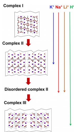
Fig. 16 Schematic of the crystal structure changes from complex I to complex II, disordered complex II and complex III. Reprinted with permission from ref. 132 copyright 2016, Elsevier.
