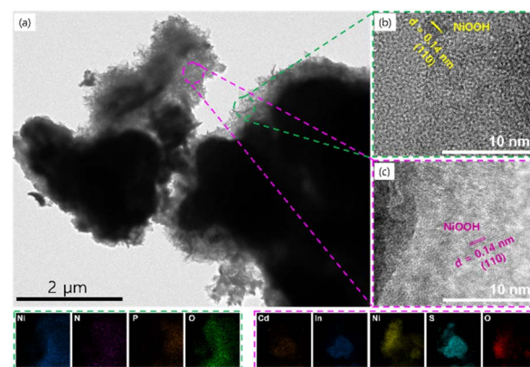
Fig. 6 (a) TEM image of the NH 4 NiPO 4 ·H 2 O/CdIn 2 S 4 /Ni 3 S 2 heterostructure after the UOR process, highlighting the overall morphology and nanoscale features. (b) HRTEM image illustrating the formation of the NiOOH phase via surface reconstruction during UOR. (c) HRTEM image illustrating the formation of the NiOOH phase via surface reconstruction during UOR. The bottom panel displays TEM elemental mappings, confirming the uniform distribution of elements within the NH 4 NiPO 4 ·H 2 O/CdIn 2 S 4 /Ni 3 S 2 heterostructure and validating the formation of NiOOH at the reconstructed regions.
