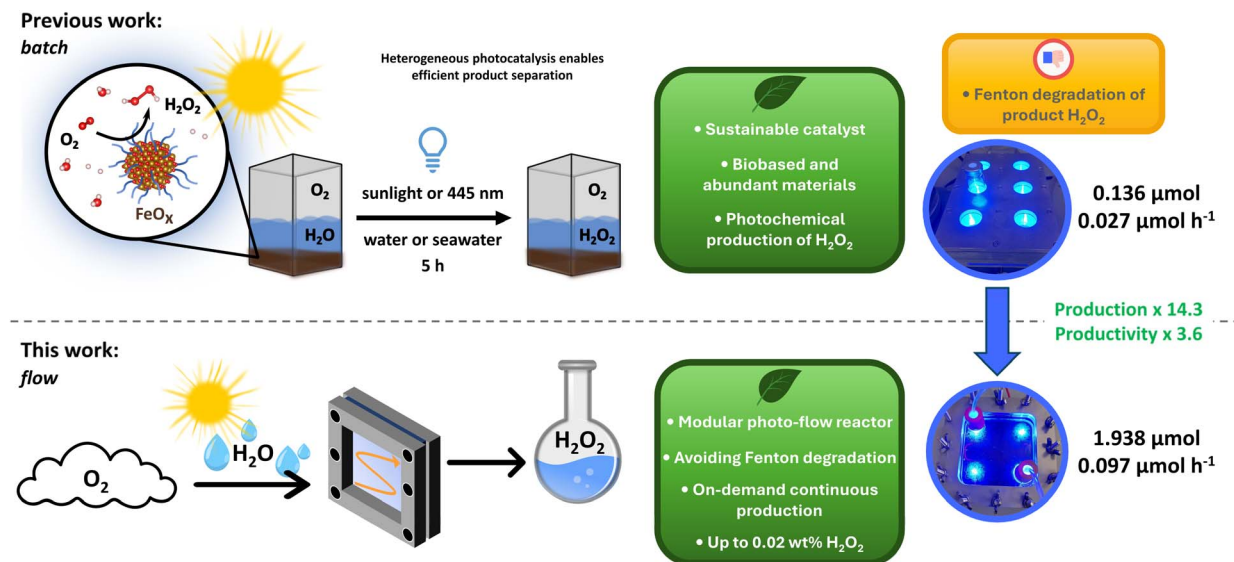
Fig. 1 Schematic representation of our previous study and the present work for photochemical production of \text{H}_2\text{O}_2 . Batch and flow conditions are compared, where flow conditions allow for higher production.
