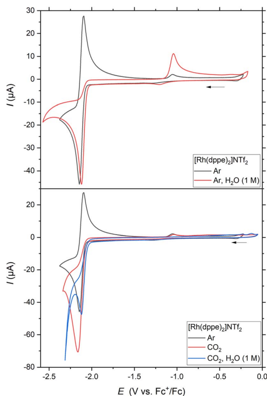
Fig. 5 Cyclic voltammograms of [\text{Rh}(\text{dppe})_2]\text{NTf}_2 . Conditions: 1\text{ mM Rh}^{\text{I}} in \text{MeCN} , 0.2\text{ M } n\text{Bu}_4\text{NPF}_6 , glassy carbon working electrode, 100\text{ mV s}^{-1} .
