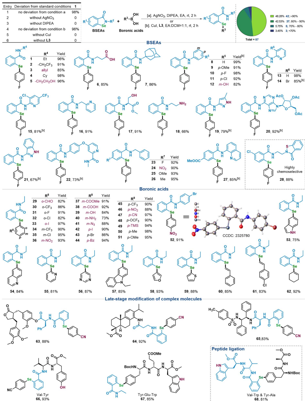
Fig. 2 Scope of the substrates. Standard conditions [a]: BSEA (0.2 mmol), boronic acid (0.24 mmol), DIPEA (0.3 mmol), and AgNO 3 (5 mol%) in EA (2 mL), rt, and 2 h (without air exclusion). Standard conditions [b]: BSEA (0.2 mmol), boronic acid (0.24 mmol), CuI (5 mol%), and L3 (5,5'-dimethyl-2,2'-bipyridine, 5 mol%) in EA : DCM = 1 : 1 (2 mL), rt, and 2 h (without air exclusion). Isolated yields are given.
