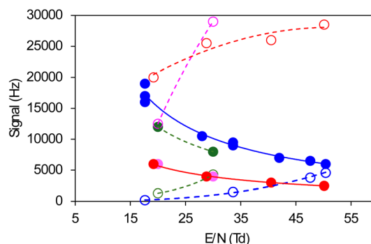
Fig. 1 Fragmentation and proton transfer channels for \text{H}_3\text{COOCH}_3 in a CIMS as a function of the ionization conditions (energy, \text{E/N} (in Td), and drift tube pressure). Open symbols = fragmentation channel monitored at m/z 31. Solid symbols = proton transfer channel, sum of m/z 81 and 99. Colors correspond to different pressures in the drift tube: blue = 20 torr; green = 15 torr; pink = 10 torr; red = 5 torr.
