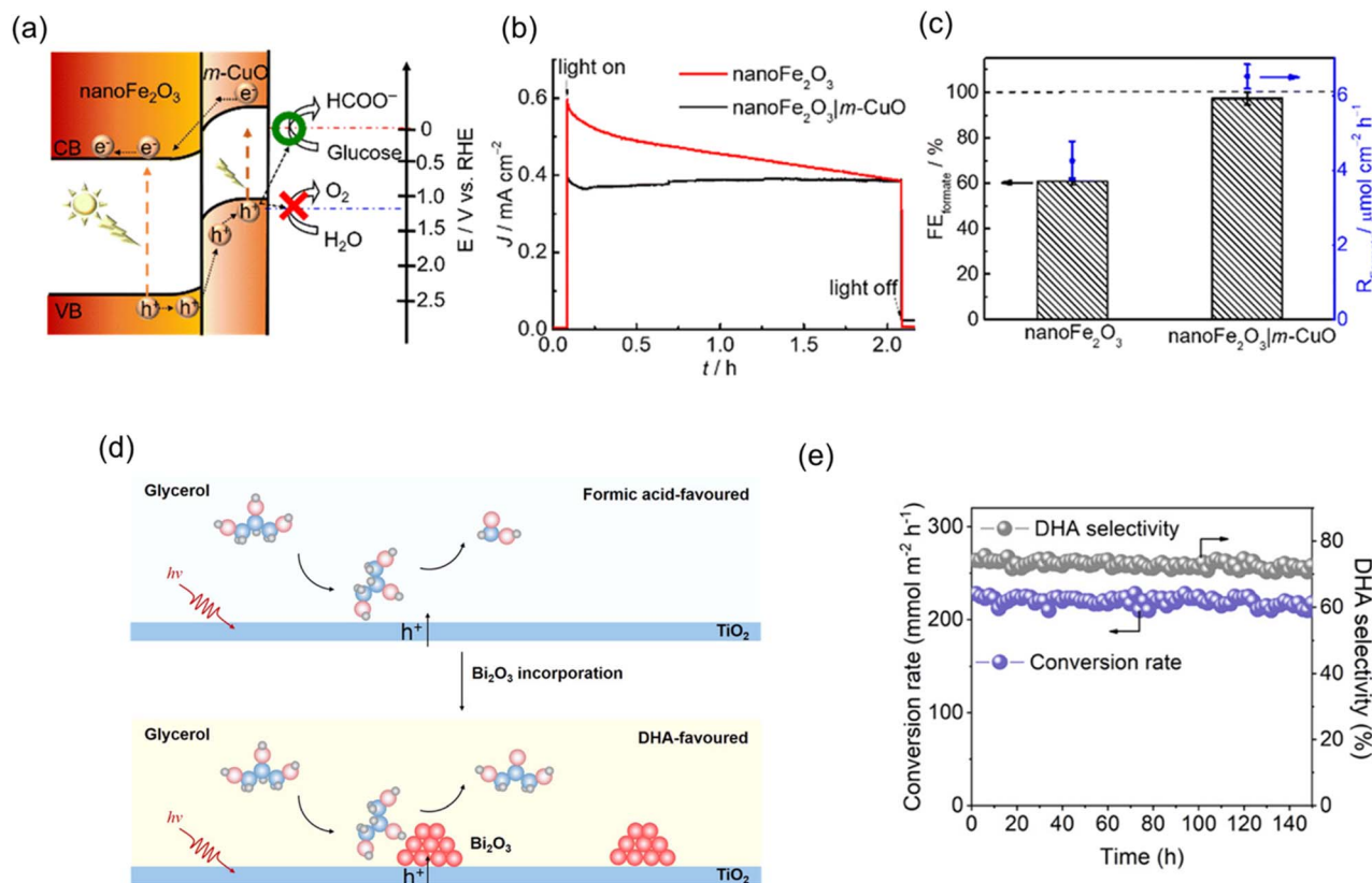
Fig. 10 (a) Band diagram of the \text{nanoFe}_2\text{O}_3/m\text{-CuO} . (b) CPE measurements of \text{nanoFe}_2\text{O}_3 and \text{nanoFe}_2\text{O}_3/m\text{-CuO} , and (c) their corresponding FE and production rate of FA in 0.1 M NaOH with 20 mM glucose under solar light irradiation (AM 1.5 G, 100 \text{ mW cm}^{-2} ). Reproduced with permission. 119 Copyright 2022, Royal Society of Chemistry. (d) Schematic of PEC glycerol oxidation over \text{TiO}_2 and \text{Bi}_2\text{O}_3/\text{TiO}_2 heterojunction and (e) long-term stability test of \text{Bi}_2\text{O}_3/\text{TiO}_2 photoanode for PEC glycerol oxidation. Reproduced with permission. 56 Copyright 2022, American Chemical Society.
