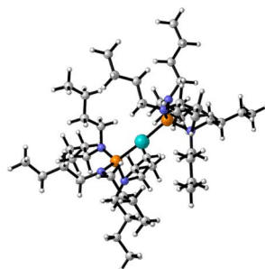
PdB 2 Two P3N ligands on Pd
