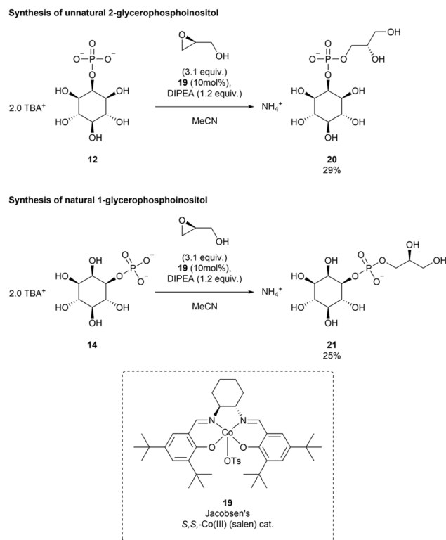
Scheme 6 Synthesis of 1-GroPIs 21 and the non-natural 2-GroPIs derivative 20 via Co(III) catalyzed epoxide ring opening of S -( S )-glycidol with InsP 1 isomers.
