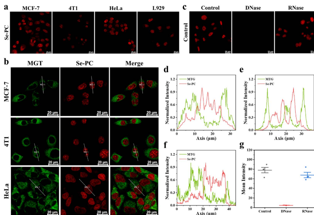
Fig. 2 (a) Confocal images of MCF-7, 4T1, HeLa and L929 cells co-stained with Se-PC ( 1 \mu\text{M} ), respectively. (b) Confocal images of MCF-7, 4T1 and HeLa cells co-stained with Se-PC ( 1 \mu\text{M} ) and MTG ( 1 \mu\text{M} ), respectively. (c) Confocal images of fixed MCF-7 cells co-stained with Se-PC ( 1 \mu\text{M} ) following treatment with DNase I ( 100 \text{ U mL}^{-1} ) or RNase A ( 100 \mu\text{g mL}^{-1} ), respectively. (d–f) Curve chart: intensity correlation of Se-PC and MTG in (b). (d) ROI of MCF-7 cells, (e) ROI of 4T1 cells and (f) ROI of HeLa cells. (g) Mean fluorescence intensity of Se-PC in (c). Scale bar: 20 \mu\text{m} .
