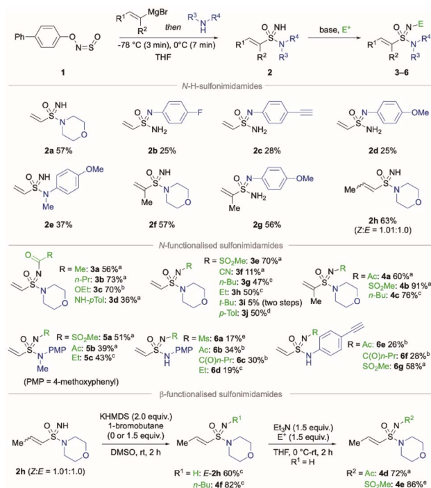
Scheme 1 Synthesis of N -H- and N -functionalised sulfonimidamides from BiPhONSO. Conditions for N -H sulfonimidamides: BiPhONSO (1.0 equiv.), alkenyl Grignard (1.0 equiv.), THF, -78^\circ\text{C} , 3 min then amine (1.2–1.5 equiv.), -78^\circ\text{C} to 0^\circ\text{C} , 7 min. Functionalization of vinylsulfonimidamides: 1.0 equiv. of sulfonimidamide was used in all cases. a Et 3 N (1.5 equiv.), E + (1.1–1.5 equiv.), THF, 0^\circ\text{C} to rt, 2–20 h; b pyridine (1.5–1.8 equiv.), E + (1.1–1.5 equiv.), THF, 0^\circ\text{C} to rt, 3–16 h; c KHMDs (2.0 equiv.), E + (0–1.5 equiv.), DMSO, rt, 2 h; d p -tolyl boronic acid (2.3 equiv.), Cu(MeCN) 4 BF 4 (15 mol%), DMF, rt, O 2 , 24 h; e NaH (1.2 equiv.), MsCl (1.1 equiv.), THF, 0^\circ\text{C} to rt, 18 h.
