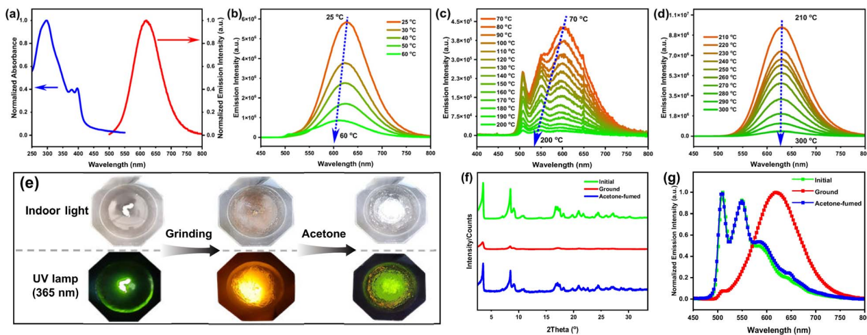
Fig. 1 Ultraviolet-visible (UV-vis) absorption and PL spectra of Pt8 in a spin-coated film (6 mg mL -1 in chloroform; 1000 rpm, 30 s) at room temperature (a); PL spectra of Pt8 after thermal annealing at different temperatures (b–d); the photos (e), XRD patterns (f) and PL switching (g) of Pt8 at the initial powder, ground and acetone fumigation states.
