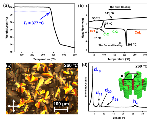
Fig. 2 TGA curve (a) and DSC traces (b) of Pt8 (at a scan rate of 10 °C min -1 under a nitrogen atmosphere); POM image (c) and XRD pattern (d) of Pt8 at 260 °C on cooling.
