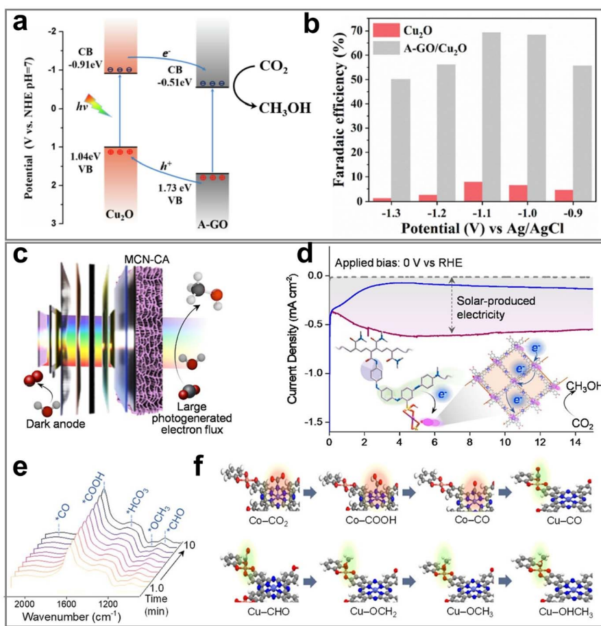
Fig. 14 (a) A schematic diagram of the charge transfer mechanism of A-GO/ \text{Cu}_2\text{O} in the PEC \text{CO}_2\text{RR} . (b) FE of \text{CH}_3\text{OH} production. Reproduced with permission from ref. 228. Copyright 2021, Elsevier B.V. All rights reserved. (c) Schematic depiction of solar \text{CH}_3\text{OH} production by the MCN photoelectrode with enhanced photogenerated electron flux. (d) Photocurrent density generated by solar irradiation of MCN-CA and MCN-C. (e) In situ FT-IR spectra of cobalt-phthalocyanine catalyst assembly. (f) Schematic illustration of the cooperative \text{CO}_2 -to- \text{CH}_3\text{OH} conversion mechanism for cobalt-phthalocyanine catalyst assembly. Reproduced with permission from ref. 212. Copyright 2024, American Chemical Society.
