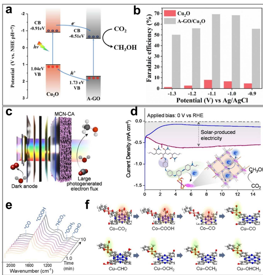
Fig. 14 (a) A schematic diagram of the charge transfer mechanism of A-GO/ \text{Cu}_2\text{O} in the PEC \text{CO}_2 RR. (b) FE of \text{CH}_3\text{OH} production. Reproduced with permission from ref. 228. Copyright 2021, Elsevier B.V. All rights reserved. (c) Schematic depiction of solar \text{CH}_3\text{OH} production by the MCN photoelectrode with enhanced photogenerated electron flux. (d) Photocurrent density generated by solar irradiation of MCN-CA and MCN-C. (e) In situ FT-IR spectra of cobalt-phthalocyanine catalyst assembly. (f) Schematic illustration of the cooperative \text{CO}_2 -to- \text{CH}_3\text{OH} conversion mechanism for cobalt-phthalocyanine catalyst assembly. Reproduced with permission from ref. 212. Copyright 2024, American Chemical Society.
