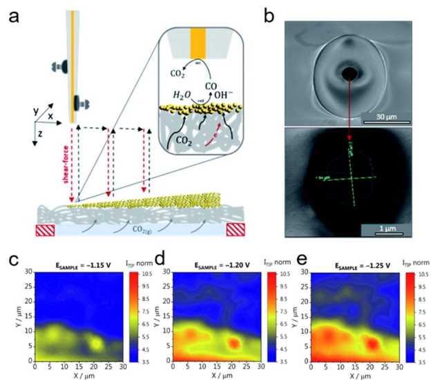
Fig. 6 (a) Schematic representation of the SECM experimental setup, with the Au UME mounted on the piezo, approaching the GDE coated with catalysts using the capacitance-based approach curve. After the Au UME was positioned near the GDE, the \text{CO}_2\text{RR} activity was characterized in the SG-TC mode, as shown in the inset. (b) SEM micrographs of the Au UME. (c–e) Activity maps recorded for the GDE at a \text{CO}_2 back-pressure of 0.7 mbar. The GDE potentials were reported versus Ag/AgCl/3 M KCl in 1 M \text{KHCO}_3 . The tip current ( I_{\text{tip}} norm) was normalized to the double-layer charging current recorded at -0.6 \text{ V} . Reproduced with permission from ref. 69, Royal Society of Chemistry, 2021.
