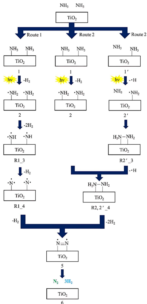
Fig. 5 Suggested reaction mechanism for \text{NH}_3 decomposition to form \text{N}_2 and \text{H}_2 over a \text{TiO}_2 photocatalyst. Reproduced from ref. 50 with permission from Elsevier, Copyright 2017.
