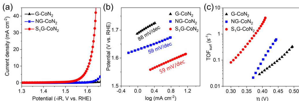
Fig. 3 (a) LSVs of G-CoN 2 , NG-CoN 2 and S 1 G-CoN 2 , 1 M KOH, 10 mV s -1 scan rate, 1600 rpm. The potentials are compensated by 95% i R loss. (b) The corresponding Tafel slopes derived from LSVs. (c) TOF surf of Co sites for catalyzing OER.
