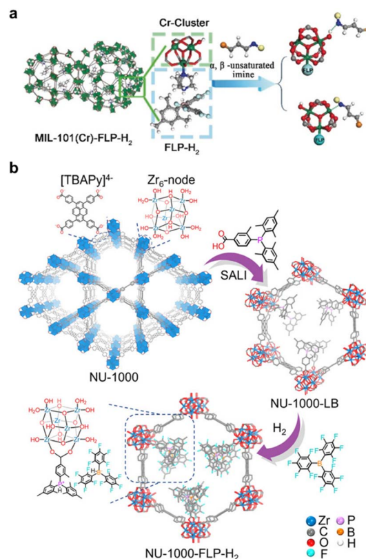
Fig. 13 (a) The "activation" process involving a \text{Cr}_3(\mu_3\text{-O})(\text{COO})_6(\text{OH})(\text{H}_2\text{O})_2 cluster in MIL-101(Cr)-FLP-H 2 . Reproduced with permission. 219 Copyright 2019, John Wiley and Sons. (b) Construction pathway of NU-1000-FLP-H 2 . Reproduced with permission. 220 Copyright 2023, American Chemical Society.
