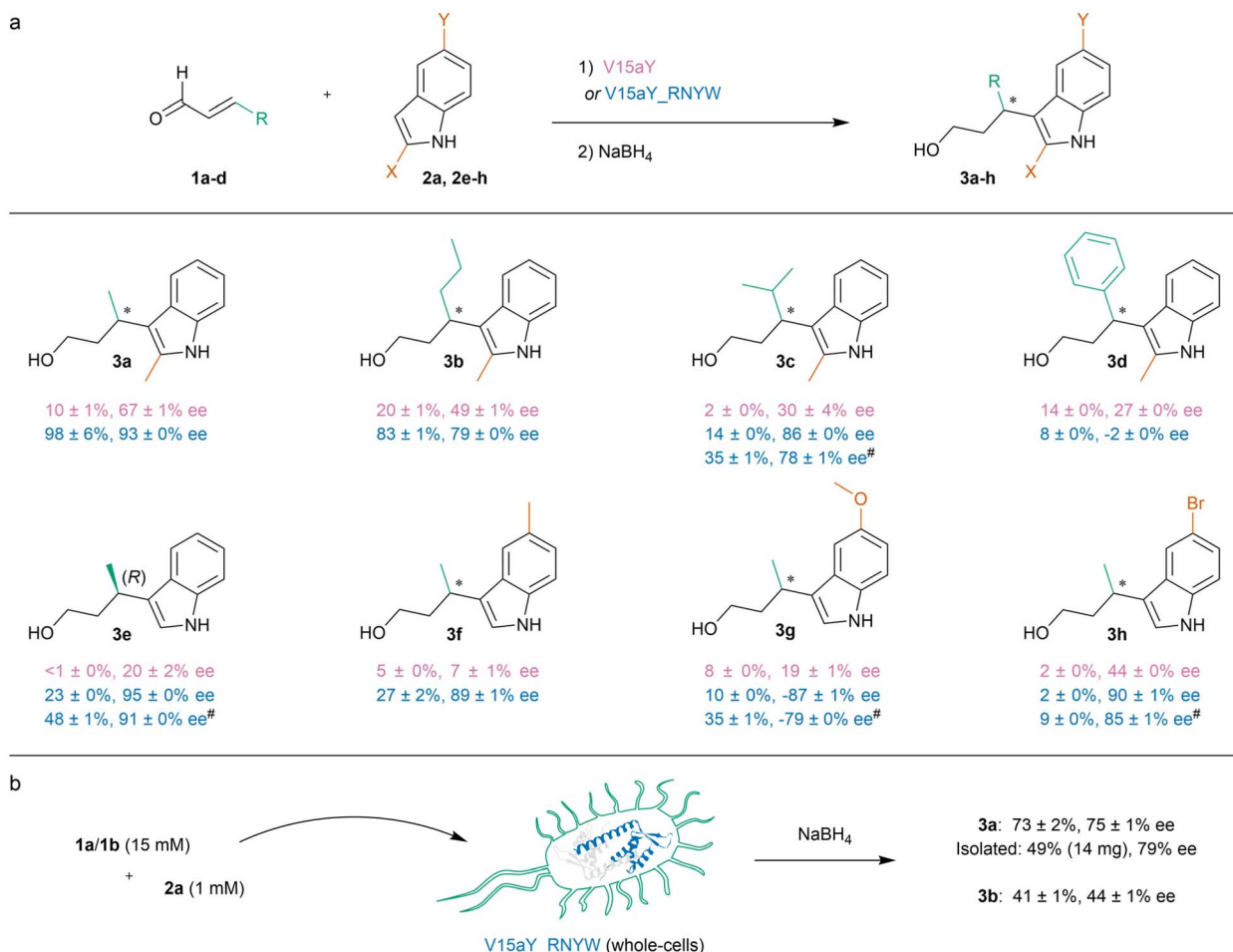
Scheme 2 (a) Substrate scope of the enantioselective vinylogous FC-alkylation reaction catalysed by V15aY and V15aY_RNYW. Reaction conditions (unless otherwise noted): V15aY variant (60 μM dimer concentration), 1a–d (5 mM), 2a, 2e–h (1 mM) in MES buffer (20 mM, pH 5.5), containing NaCl (150 mM) and DMF (8% v/v) in a total volume of 300 μL, continuously inverted for 16 h at 8 °C. For 3a–d and 3f–h , ee is assigned relative to the enantiomer obtained with V15aY, in which the “–” symbol represents the opposite enantiomer. For 3e , absolute configuration is assigned by comparison of order of elution on HPLC with the literature and previous work. 16,42 # Performed using 25 mM 1 , see Table S5† for results of reactions performed at 25 °C. (b) Whole-cell catalysis and application on millimolar scale. Reaction conditions: washed whole-cells expressing V15aY_RNYW (6 OD 600 units), 1a/1b (15 mM), 2a (1 mM) in MES buffer (20 mM, pH 5.5), containing NaCl (150 mM) and DMSO (8% v/v) in a total volume of 300 μL, continuously inverted for 21 h at 8 °C. Results are based on at least three experiments, using two or more independently produced batches of protein, or three independent cultures of whole-cells. Errors are the standard deviation of the results. See ESI† sections 9 and 11 for more details.
