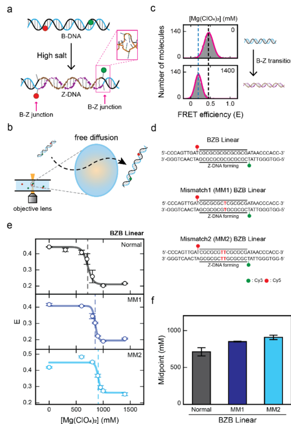
Fig. 1 Observing the effect of a mismatch in the CG repeat region for Z-DNA formation by single-molecule FRET measurement. (a) Illustration of the B–Z transition in the linear dsDNA that consists of a Z-DNA forming region that is flanked by two random sequences at both ends. Z-DNA formation is accompanied by two B–Z junctions with an extruded base pair (pink rectangle, PDB code 2ACJ). (b) Brief schematic illustration of the ALEX measurement, which detects the FRET efficiency of freely diffusing single molecules that pass through the confocal excitation volume. (c) The FRET histograms of the linear dsDNA undergoing the B–Z transition. The low-FRET peak represents Z-DNA and the high-FRET peak represents B-DNA of the BZB linear sample. (d) DNA sequences used for the experiments. The BZB linear sample consists of the CG repeat, a Z-DNA forming region, with two random sequences at both ends. Mismatched base pairs are substituted within the CG repeat region and indicated in red color. Cy3 and Cy5 were used as a FRET pair. (e) The average FRET efficiency ( E ) of each linear dsDNA sample (BZB linear, MM1 BZB linear, and MM2 BZB linear) plotted against the concentration of \text{Mg}(\text{ClO}_4)_2 . The dotted lines denote the midpoint of each sample. Error bars were obtained from three independent measurements. (f) B–Z transition midpoints for each sample were obtained from (e). As the number of the mismatches in the CG repeat increases, the B–Z transition midpoint increases. Error bars were obtained from three independent measurements.
