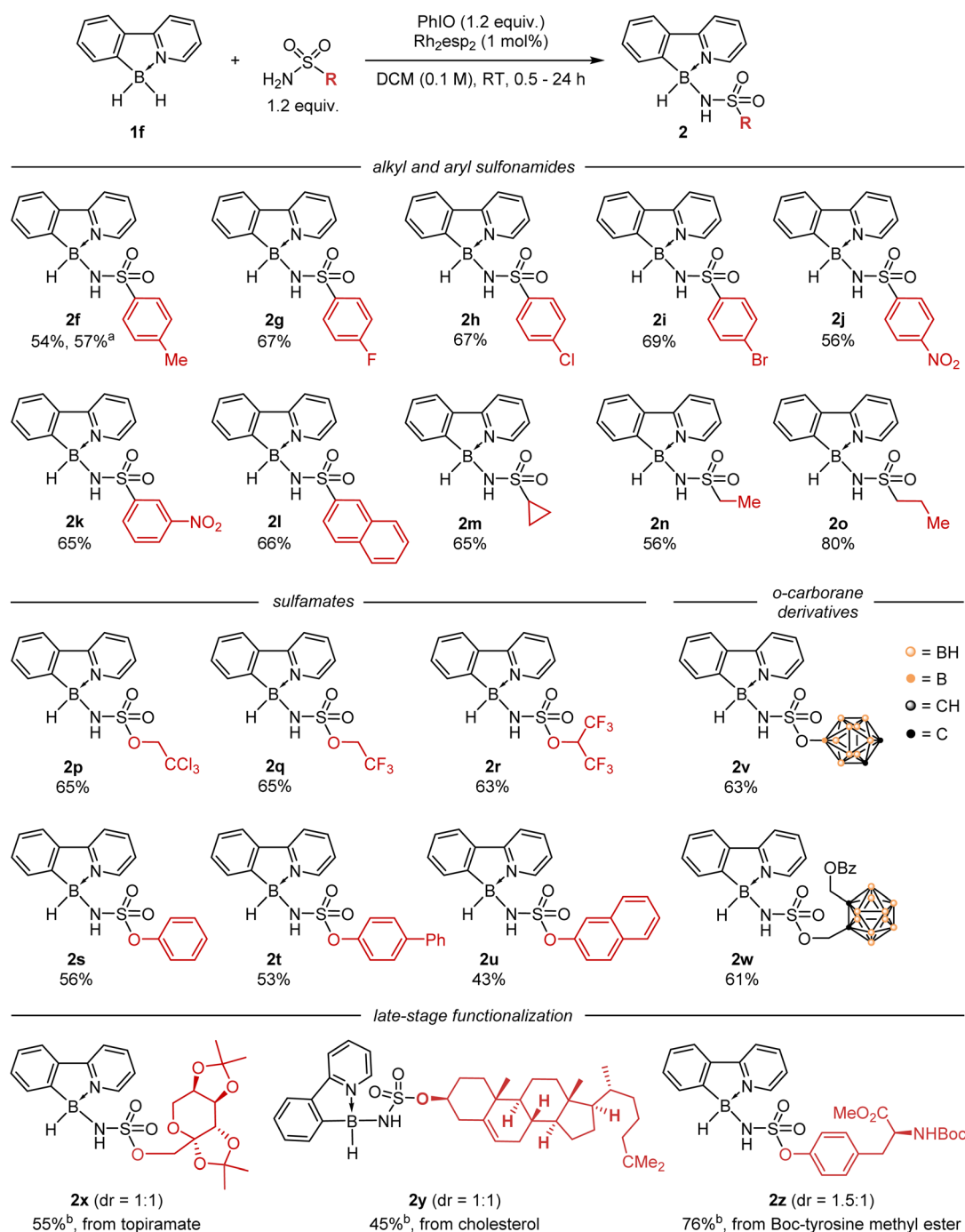
Scheme 2 Catalytic insertion of nitrenes derived from sulfonamides and sulfonates into 2-phenylpyridine–borane 1f . Reaction conditions: 1f (0.2 mmol), sulfonamide or sulfonate (0.24 mmol), PhIO (0.24 mmol), Rh 2 esp 2 (1 mol%), DCM (2 ml), RT, 0.5 to 24 h. Isolated yields are given. a Performed on a 6 mmol scale. b Performed on a 0.1 mmol scale.
