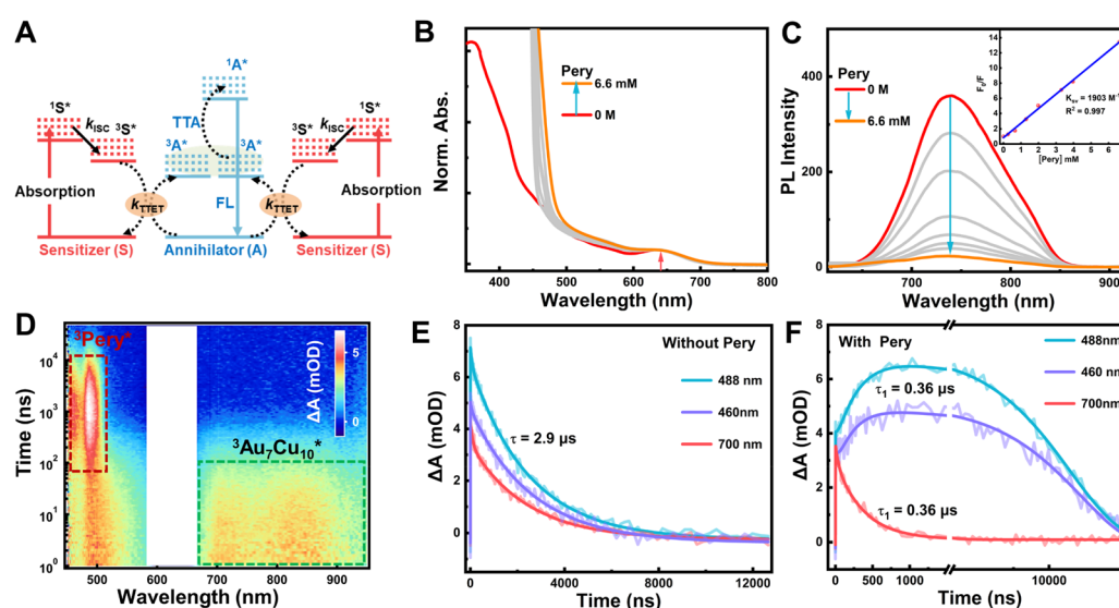
Fig. 2 (A) Schematic energy-level diagram of TTA-UC. Steady-state (B) absorption and (C) emission spectra (excitation at 600 nm) of \text{Au}_7\text{Cu}_{10} NCs in the presence of Pery. The inset of (C) shows the Stern–Volmer plot with the dynamic quenching rate constant K_{SV} . (D) ns-TA color maps of \text{Au}_7\text{Cu}_{10} /Pery dissolved in deaerated THF with 630 nm excitation; the Pery concentration was set at 3 mM. (E) The kinetic traces of \text{Au}_7\text{Cu}_{10} in THF. (F) The kinetic traces of \text{Au}_7\text{Cu}_{10} /Pery in THF with 630 nm excitation.
