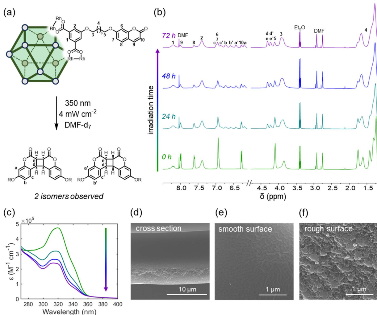
Fig. 3 (a) Irradiation of C 10 -Coumarin-RhMOP at 350 nm results in the dimerization of their side chains. (b) 1 H NMR spectra of a 5 mM DMF- d 7 solution of C 10 -Coumarin-RhMOP after irradiation at 350 nm for 0 h (green), 24 h (teal), 48 h (blue), and 72 h (purple) reveal the emergence of two correlated sets of aromatic and alkyl signals, suggesting the formation of two coumarin dimer isomers. Note that the absolute stereochemical configurations of the dimer isomers corresponding to each set of correlated peaks cannot be verified by this technique, and are therefore assigned arbitrarily. (c) UV-Vis spectra of the MOP solution at each irradiation time point reveal a decrease in the coumarin \pi \rightarrow \pi^* peak at 320 nm, corroborating the formation of cyclobutane dimers. (d–f) SEM images of the (d) cross section, (e) smooth surface, and (f) rough surface of a photopolymerized C 10 -Coumarin-RhMOP thin film produced via 350 nm irradiation of a 20 mM DMF solution of the cage.
