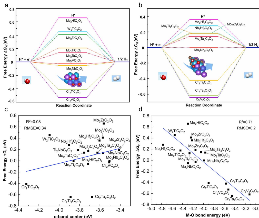
Fig. 5 (a and b) HER free energy diagrams of M'_2M''_2C_2O_2 and M'_2M''_2C_3O_2 under standard conditions, respectively. (c and d) Relationships between \Delta G_H and descriptors including (c) the p-band center of the oxygen functional group and (d) the bond energy between the first-layer transition metal and oxygen of different MXene systems, respectively.
