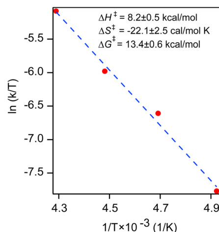
Fig. 5 Eyring analysis data showing the dependence of \ln(k/T) on 1/T for the reaction between a 50 \mu M solution of [(ArO - )(TPP)Fe III (O 2 2- )] 2- and acetophenone oxime at -40, -50, -60 and -70 °C. Solvent = 9 : 1 DCM : THF.
