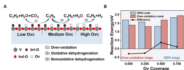
Fig. 3 Three distinct reaction stages determined by surface Ovc (A). Plot of different Ovc surfaces against the second C–H bond activation reaction energy of the C 3 H 6 * route and CH 3 O*CH 3 route (B).
