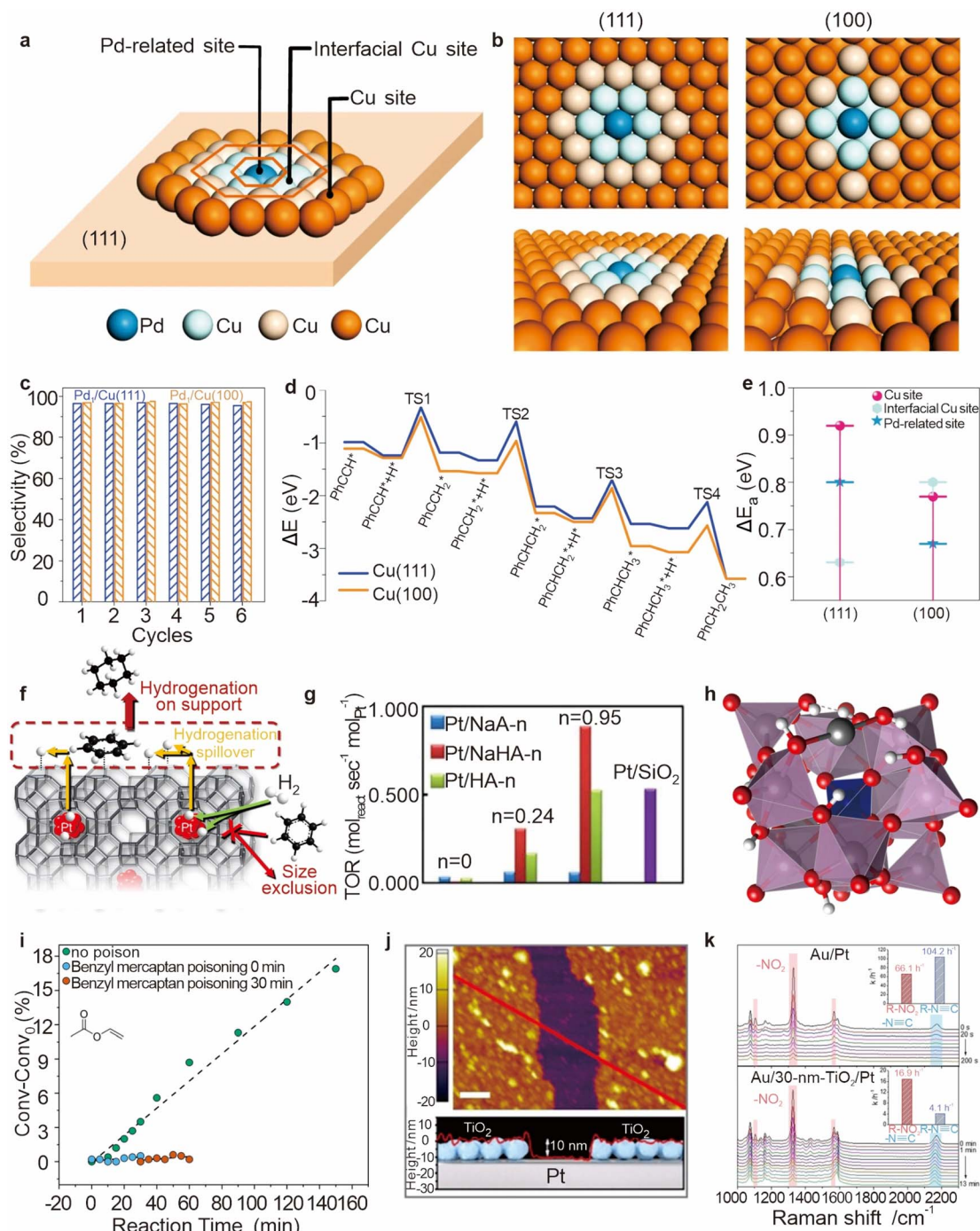
Fig. 13 (a) Three kinds of possible reactive sites on the \text{Pd}_1/\text{Cu} surface. (b) Top and side views of the \text{Pd}_1/\text{Cu}(111) and \text{Pd}_1/\text{Cu}(100) surface models. (c) Catalytic durability of \text{Pd}_1/\text{Cu}(111) and \text{Pd}_1/\text{Cu}(100) in the semi-hydrogenation of \text{PhC}\equiv\text{CH} . (d) Calculated barriers for stepwise hydrogenation of \text{PhC}\equiv\text{CH} on the two low-Miller-index Cu surfaces. (e) Calculated barriers for TS1 over different active sites on different \text{Pd}_1/\text{Cu} catalysts. Reproduced from ref. 117. Copyright 2020 Springer Nature. (f) Pt encapsulated in a dense support matrix that allows selective diffusion of hydrogen over organic reactants. (g) Turnover rates in benzene hydrogenation. Reproduced from ref. 9. Copyright 2014 Springer Nature. (h) Structure of \text{PMo}_{11}\text{O}_{39}\text{Pd}_1\text{-H}_{16} . (i) Reaction kinetics for the hydrogenation of VA with the addition of 2 equivalents benzyl mercaptan after different reaction times. Reproduced from ref. 118. Copyright 2022 Wiley-VCH GmbH. (j) AFM image of the \text{TiO}_2 nanoparticle monolayer assembled on a smooth Pt film ( \text{TiO}_2/\text{Pt} ). (k) In situ SERS spectra of the selective hydrogenation of \text{R-NO}_2 in the presence of \text{R-N}\equiv\text{C} on \text{Au}/\text{Pt} and \text{Au}/30\text{ nm-TiO}_2/\text{Pt} , respectively. Reproduced from ref. 53. Copyright 2020 Wiley-VCH GmbH.
