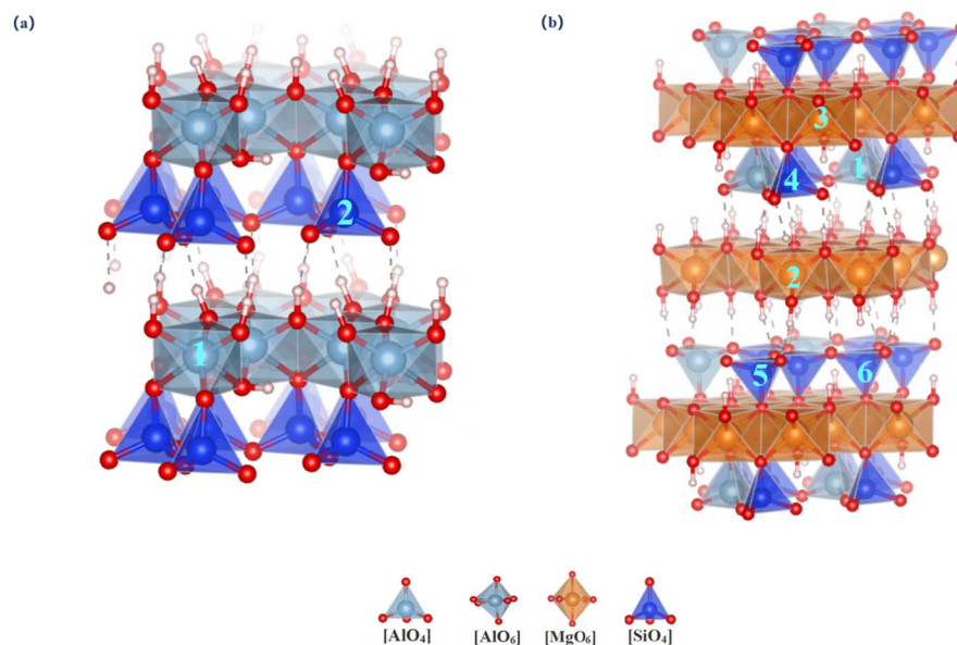
Fig. 2 Substitution site of vanadium in non-mica-type minerals [(a)-kaolinite(1-[Al vi ] 2-[Si iv ]) (b)-chlorite(1-[Al vi ] 2-[Mg vi ] 1 3-[Mg vi ] 2 4-[Si iv ] 1 5-[Si iv ] 2 6-[Si iv ] 3 )].
