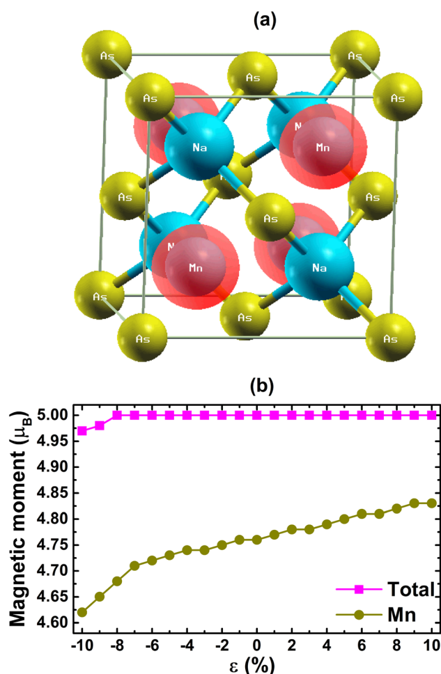
Fig. 4 (a) Spin density (iso-surface value: 0.1 \text{ e } \text{\AA}^{-3} ) at an unstrained state and (b) total magnetic moment of the NaMnAs half-Heusler compound and local magnetic moment of the Mn atom under the effects of external strain.
