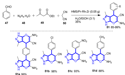
Scheme 11 Scheme for the synthesis of ( R )-6-amino-3-methyl-4-phenyl-1,4-dihydropyrano[2,3- c ]pyrazole-5-carbonitrile.
